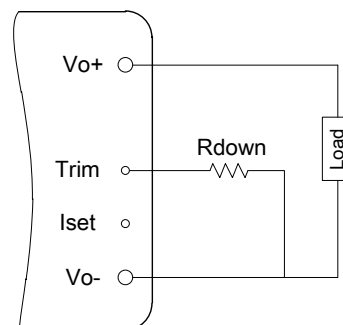
Figure 4. Circuit to Decrease Output Voltage
